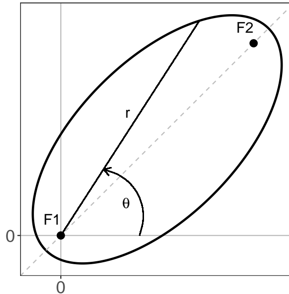
Figure 8: Sample ellipse with F_1 located at the origin
