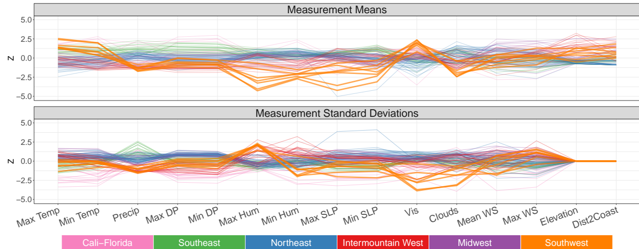
Figure 3: Parallel coordinate plot of the means and standard deviations of the weather variables listed in Table 1. Each line in the plot represents one of the 113 weather stations. The color of the lines match the weather region to which the station belongs. An interactive app is available that allows for better identification of regional trends. The Southwest region is highlighted in this graph to emphasize its weather characteristics
