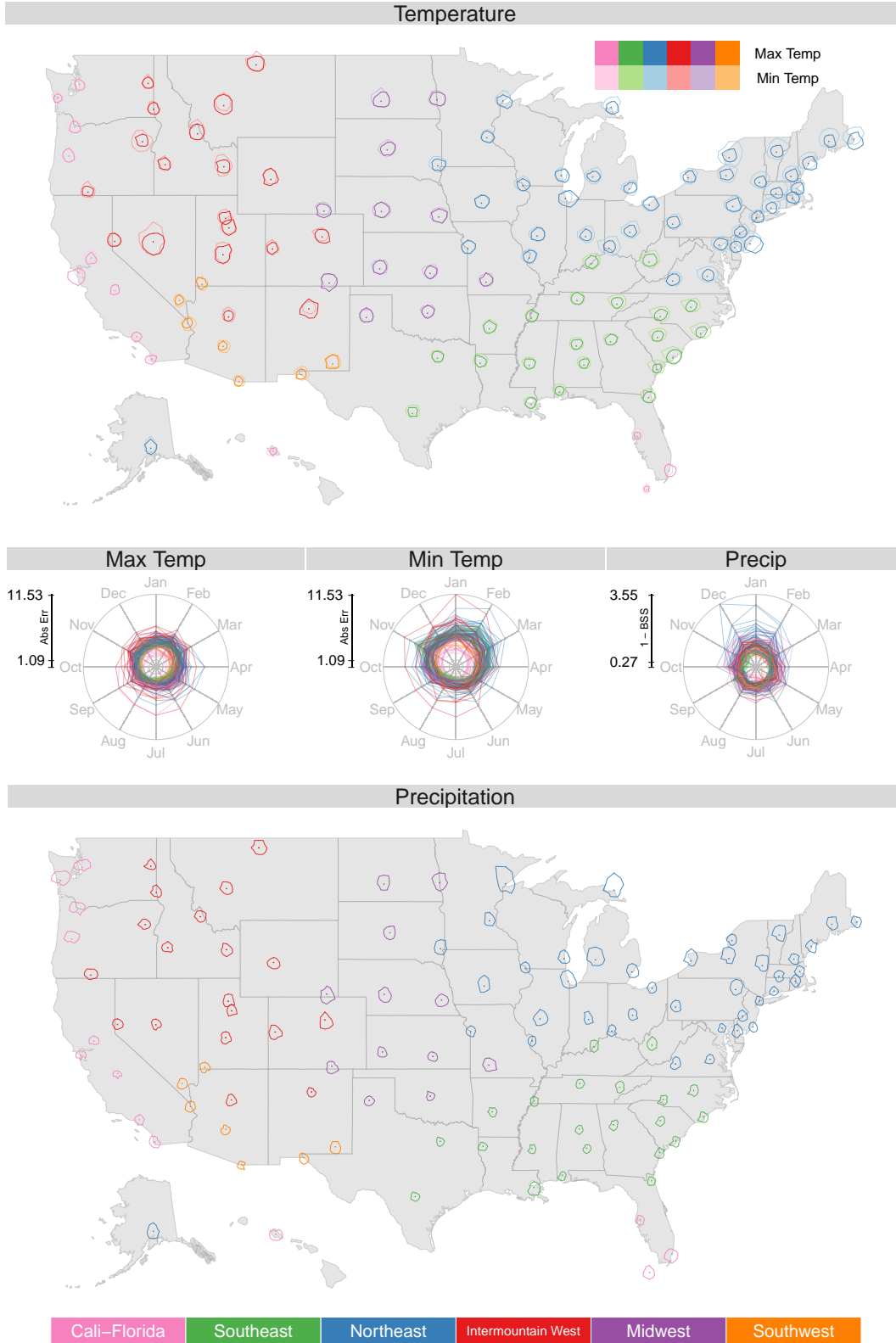
Figure 6: Glyph plots of weather forecast accuracy averaged by month. The error is represented as the scaled distance from a center point to the edge of a polygon beginning with January at the 12:00 position and proceeding clockwise
