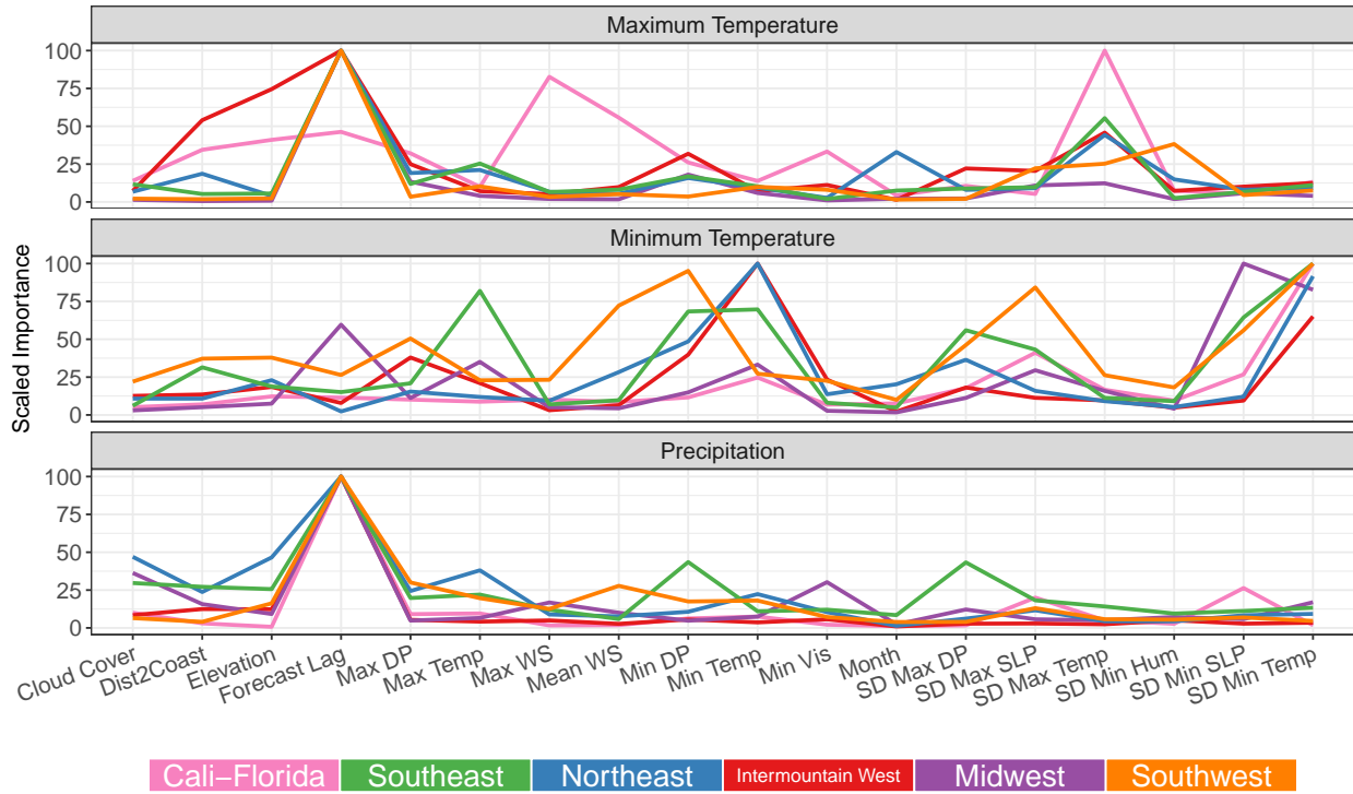
Figure 7: Variable importance for each of the three forecast accuracy measurements. Variable importance measures have been rescaled to make the measures directly comparable between weather regions and accuracy measures
